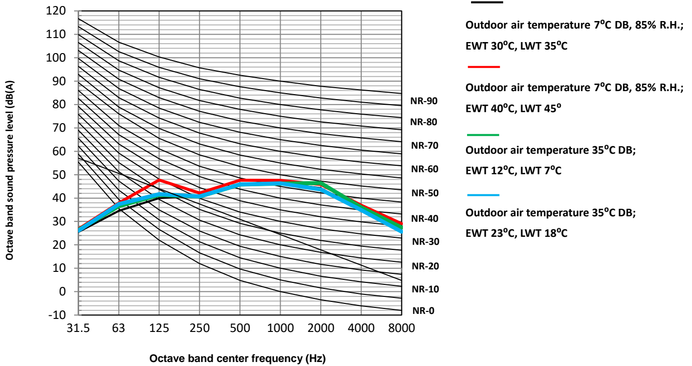
Figure 2-7.5: MDVA-V12WD2ER8-A octave band levels
