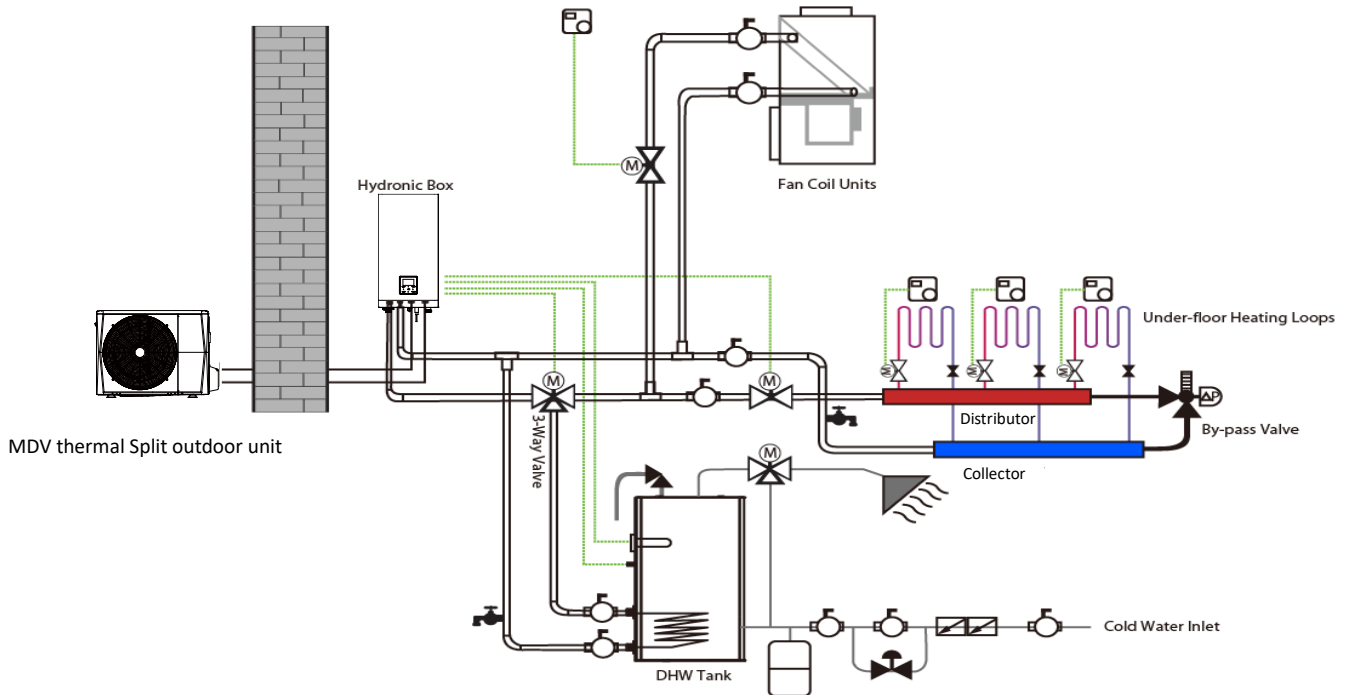
Figure 1-1.1: System schematic
