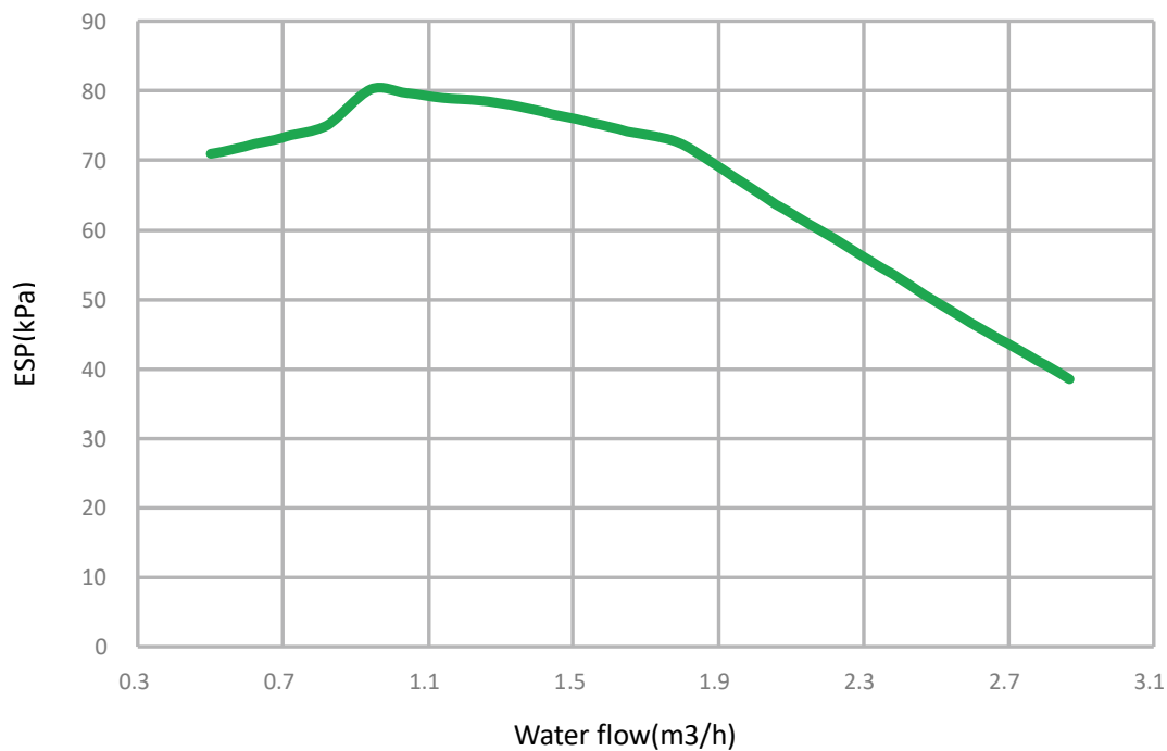
Figure 2-6.2: MDVHB-160CEGR8-A hydronic performance
