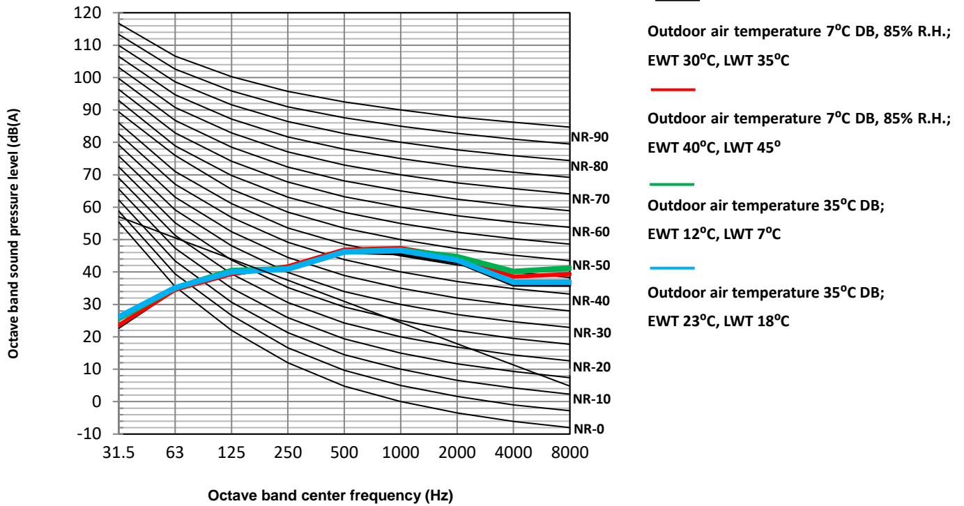
Figure 2-7.5: MDVA-V12WD2BR8-A octave band levels
