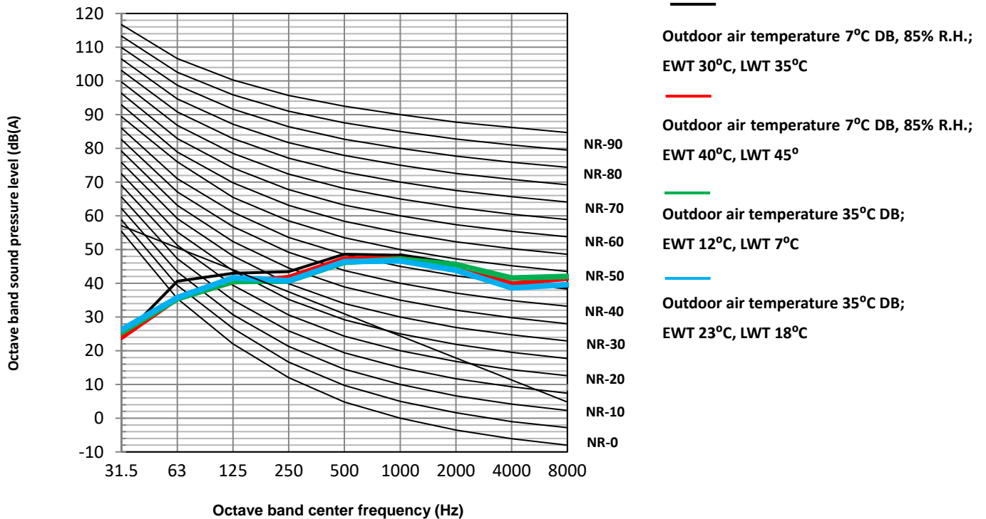
Figure 2-7.5: MDVA-V14WD2BR8-A octave band levels
