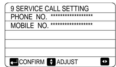
Figure 3-8.30: SERVICE CALL menu
