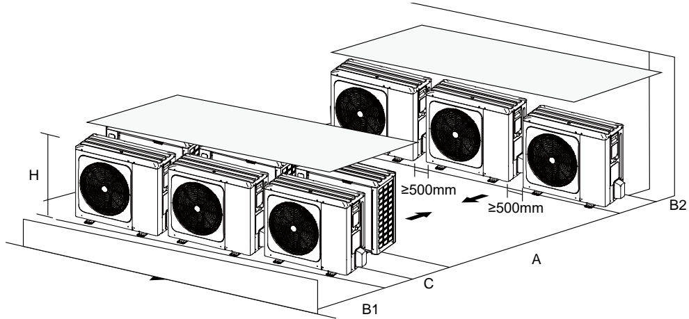
Figure 3-2.11: Multi-row installation
