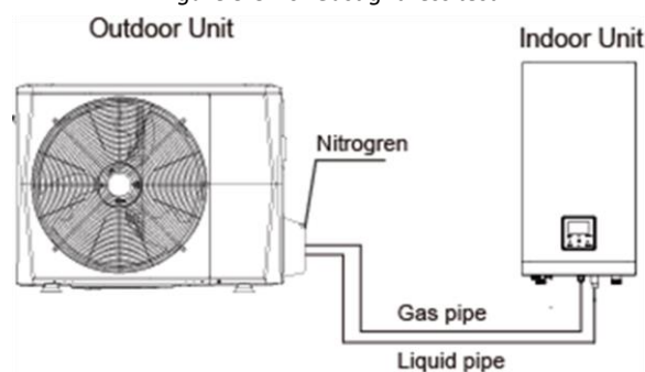
Figure 3-3.10: Gastightness test
