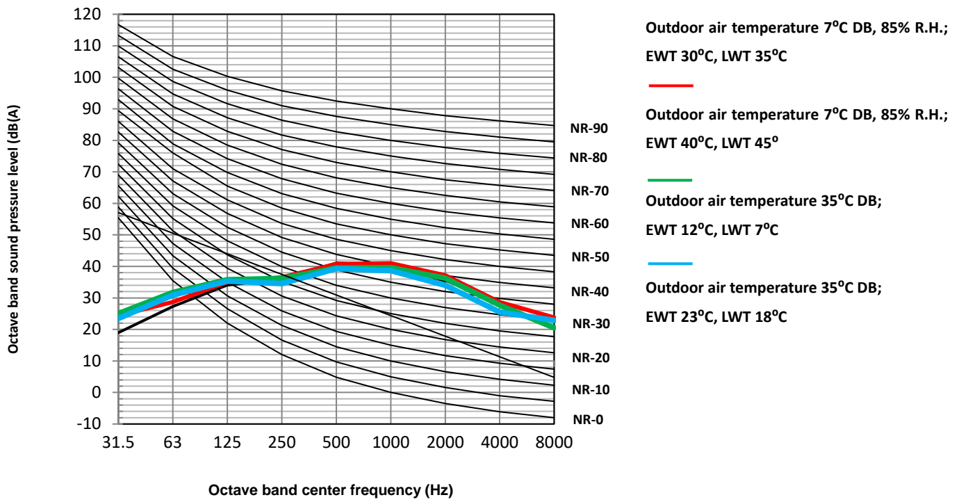
Figure 2-7.2: MDVA-V4WD2ER8-A octave band levels
