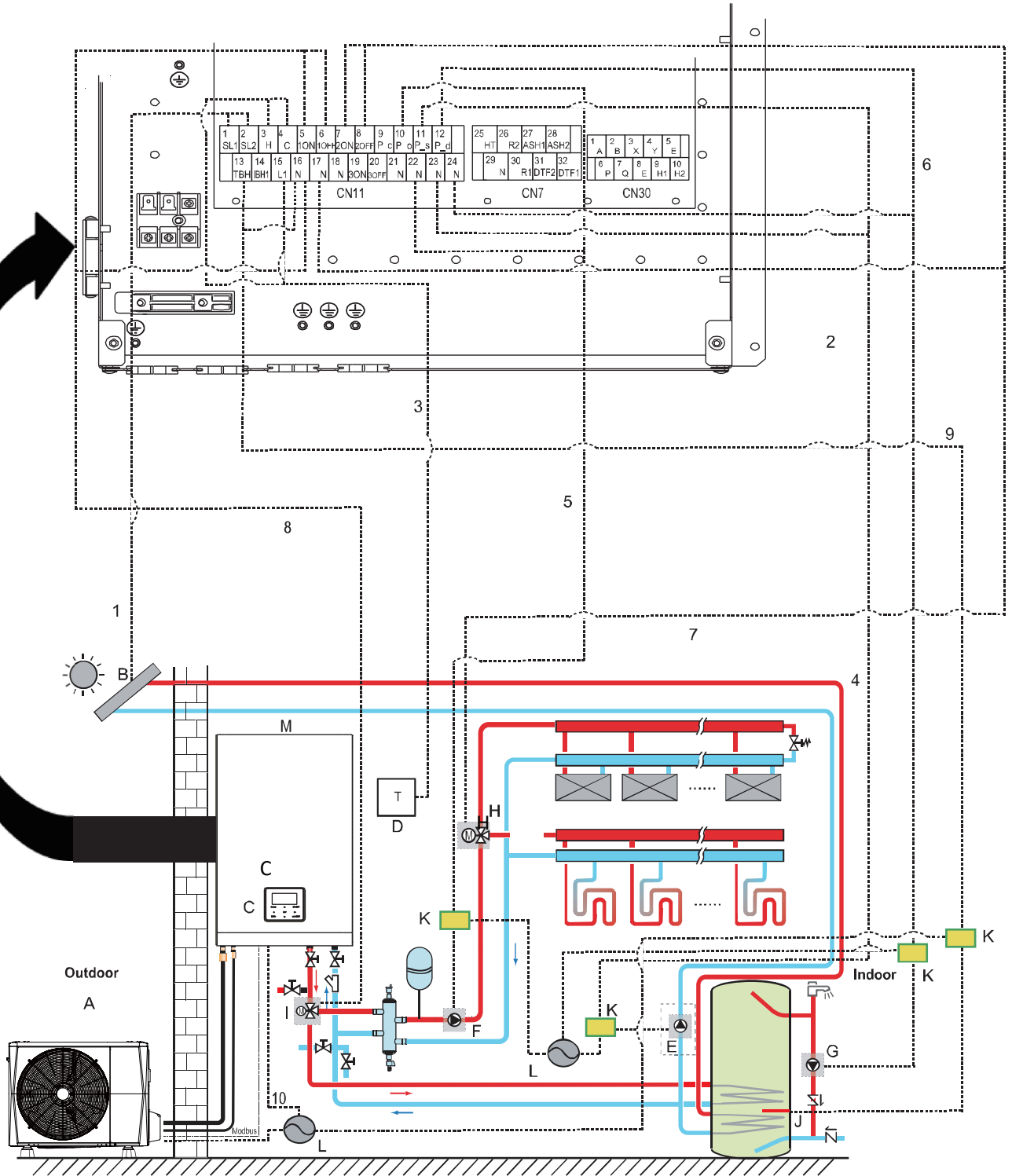
Figure 3-5.1: Wiring overview
