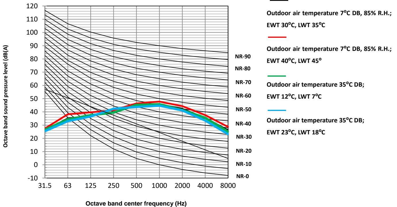
Figure 2-7.5: MDVA-V10WD2ER8-A octave band levels
