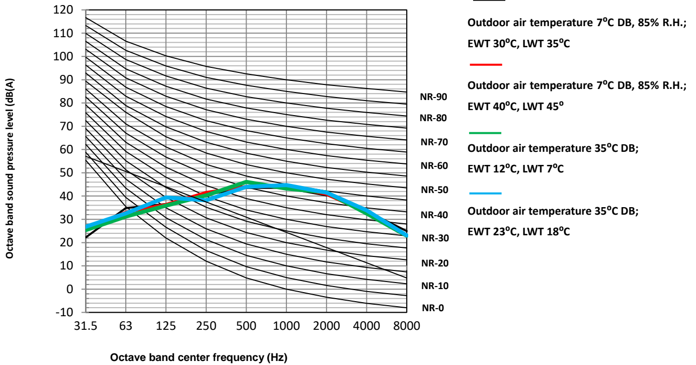
Figure 2-7.4: MDVA-V8WD2ER8-A octave band levels
