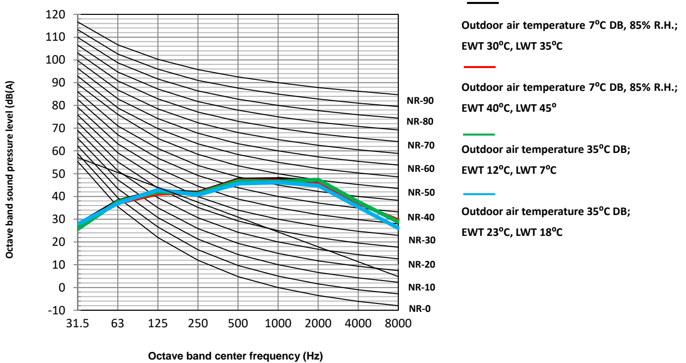
Figure 2-7.5: MDVA-V14WD2ER8-A octave band levels
