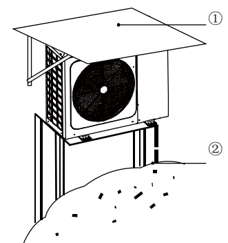
Figure 3-2.2: Snow shielding
