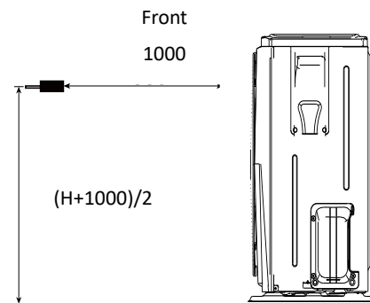
Figure 2-6.1: Sound pressure level measurement (unit: mm)
