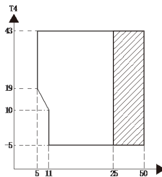
Figure 2-4.2: Cooling operating limits
