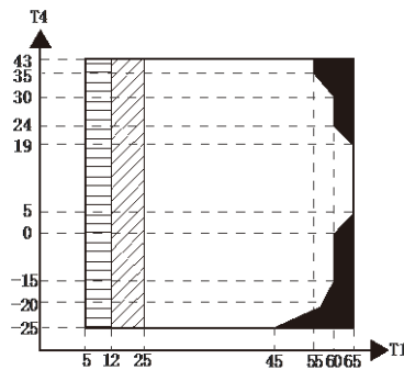
Figure 2-5.3: Domestic hot water operating limits 1
