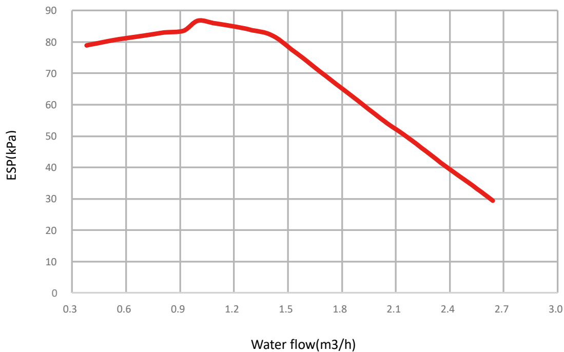
Figure 2-6.2: MDVHB-160CEGR8-A hydronic performance
