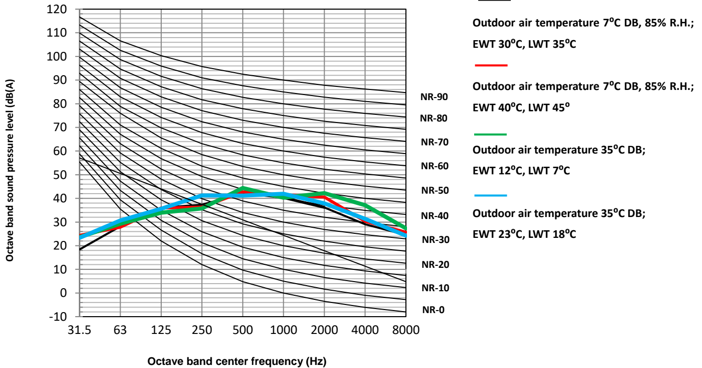
Figure 2-7.3: MDVA-V6WD2ER8-A octave band levels
