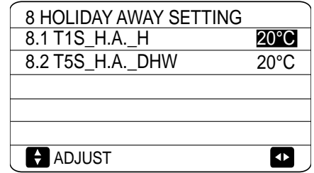
Figure 3-8.29: HOLIDAY AWAY SETTING menu
