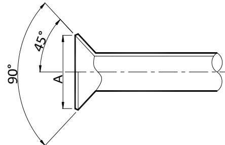
Figure 3-3.3: Flared opening
